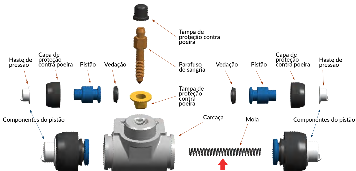
Vista explodida
